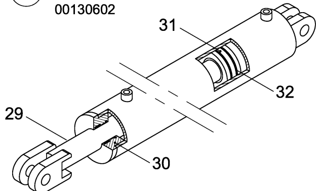
Heben / Lifting
