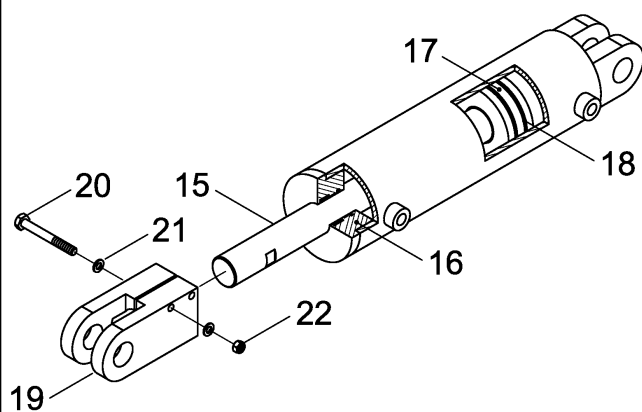
Achse / Axle
